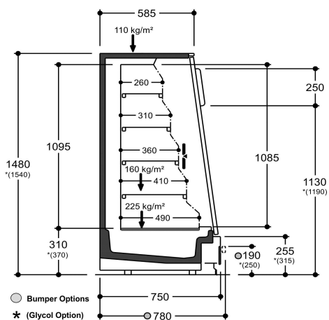
GranValdaj 15 C Tilted Doors
