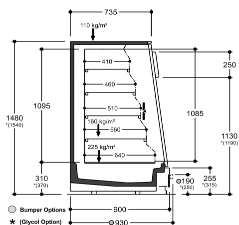
GranValdaj 15 N Tilted Doors
