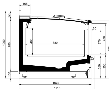
GranDrake Sliding - EOL
