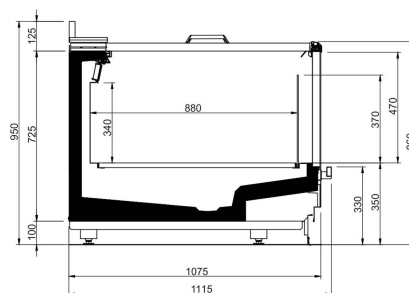
GRANDRAKE ERGO SLIDING COVERS END OF LINE
