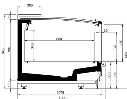
GRANDRAKE ERGO SLIDING COVERS LINEAR
